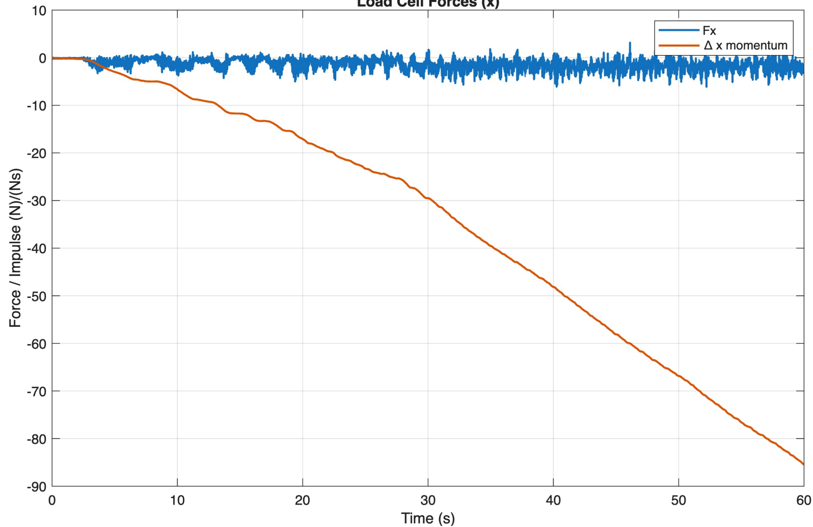
Load Cell Forces (x)
