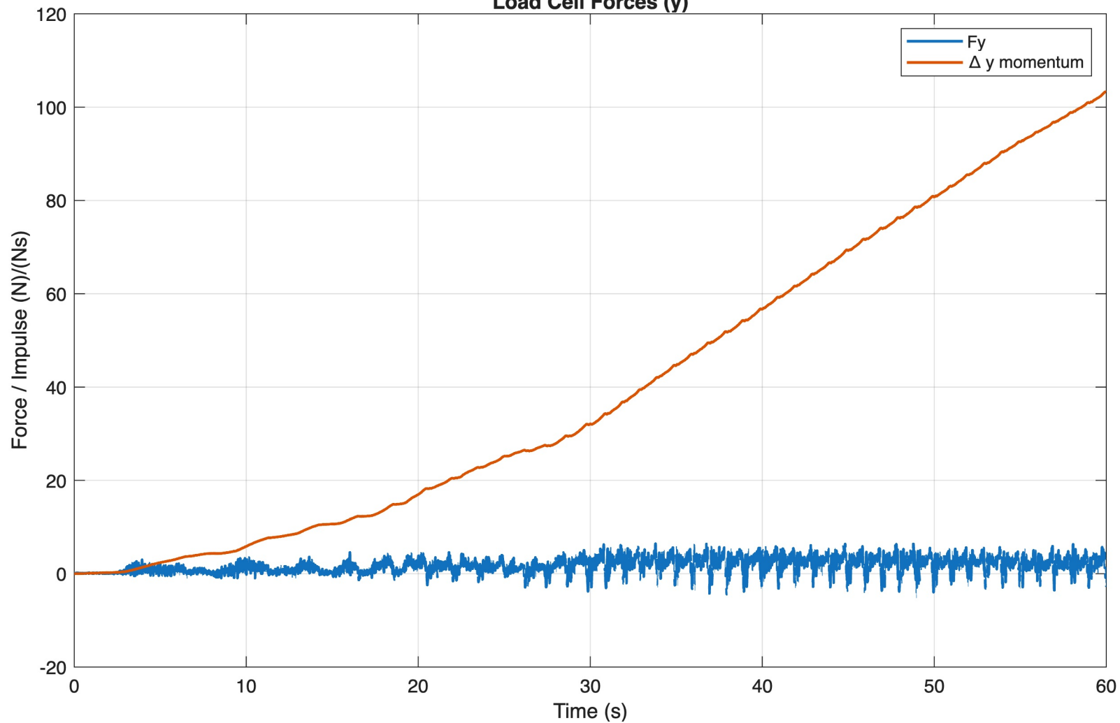
Load Cell Forces (y)
