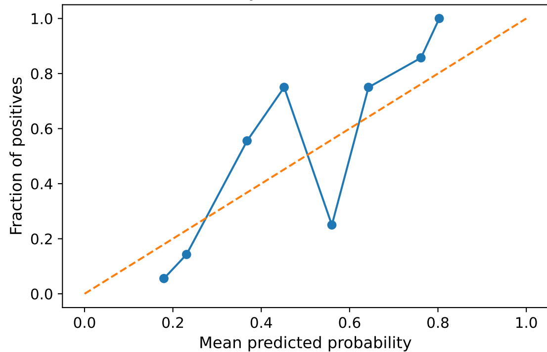
Reliability curve (Brier=0.154)
