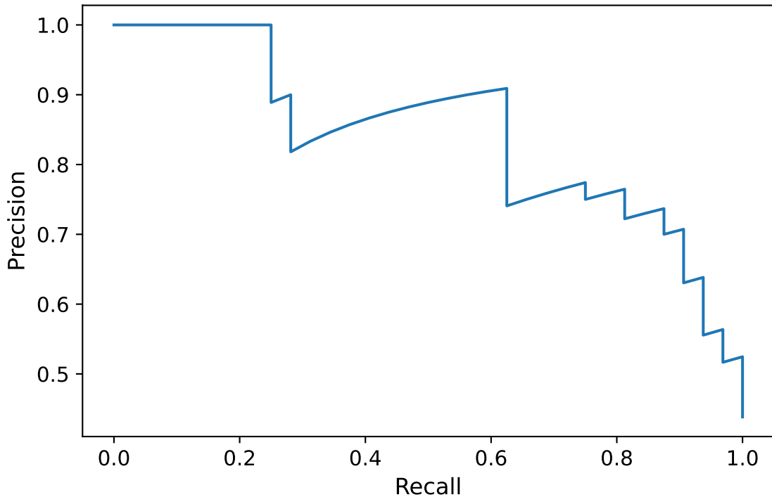
Hard-risk Precision-Recall (AP=0.845)
