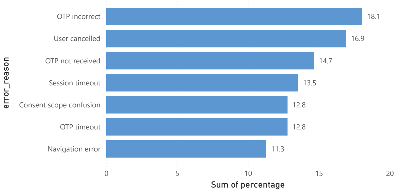
Sum of percentage by error_reason
