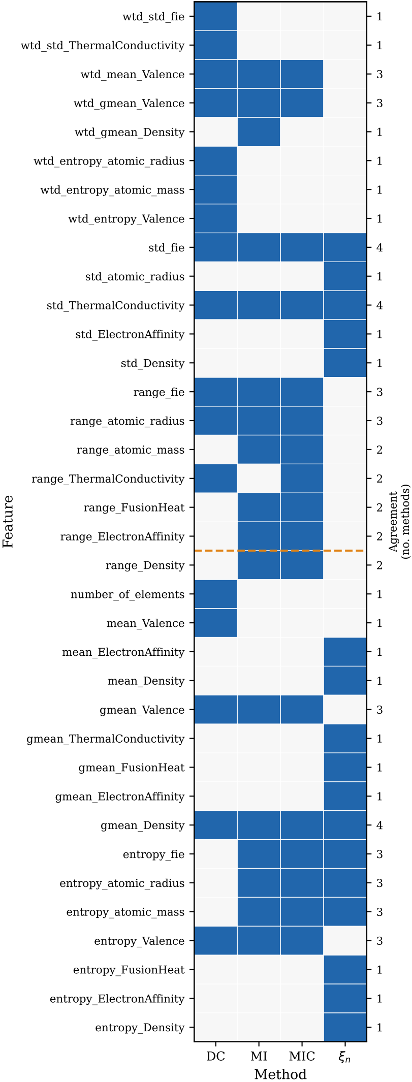
Complete feature selection agreement matrix (36 descriptors, 20\% threshold)
