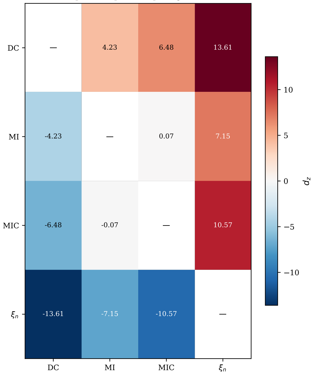
(b) Cohen's d_z (Exp. \sim 2 , 30 paired reps, LightGBM)
