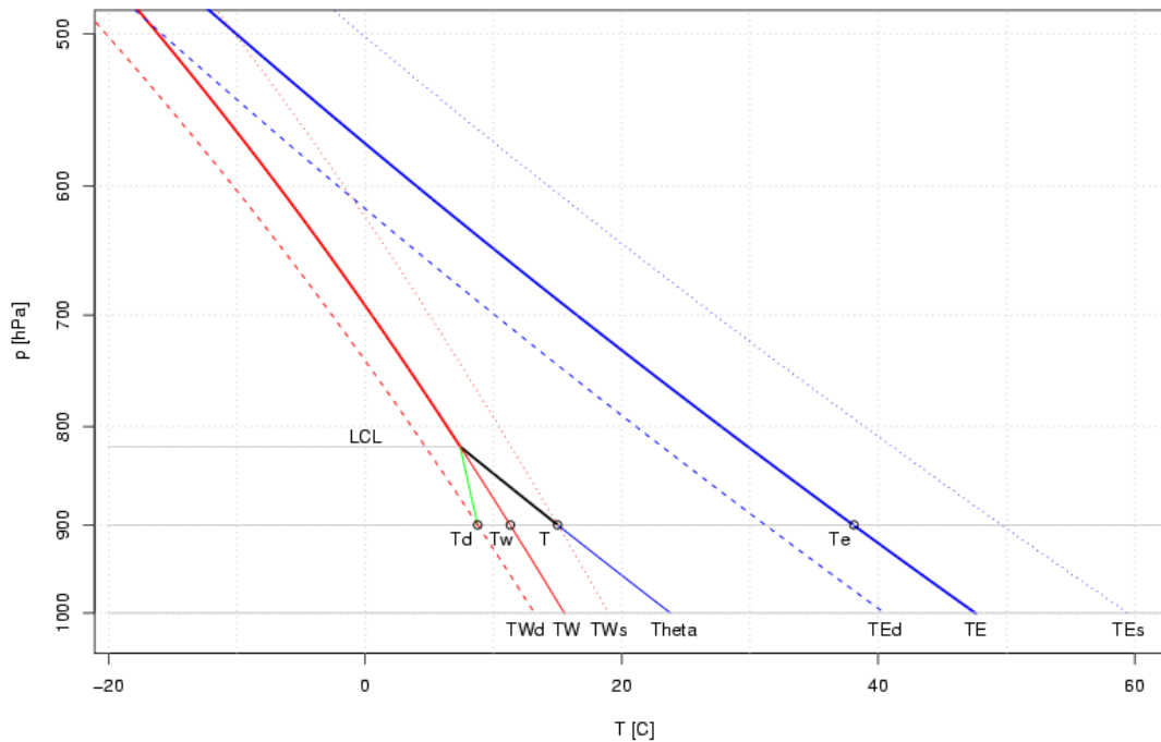
Adiabatic lifting of a parcel and some variable definitions
