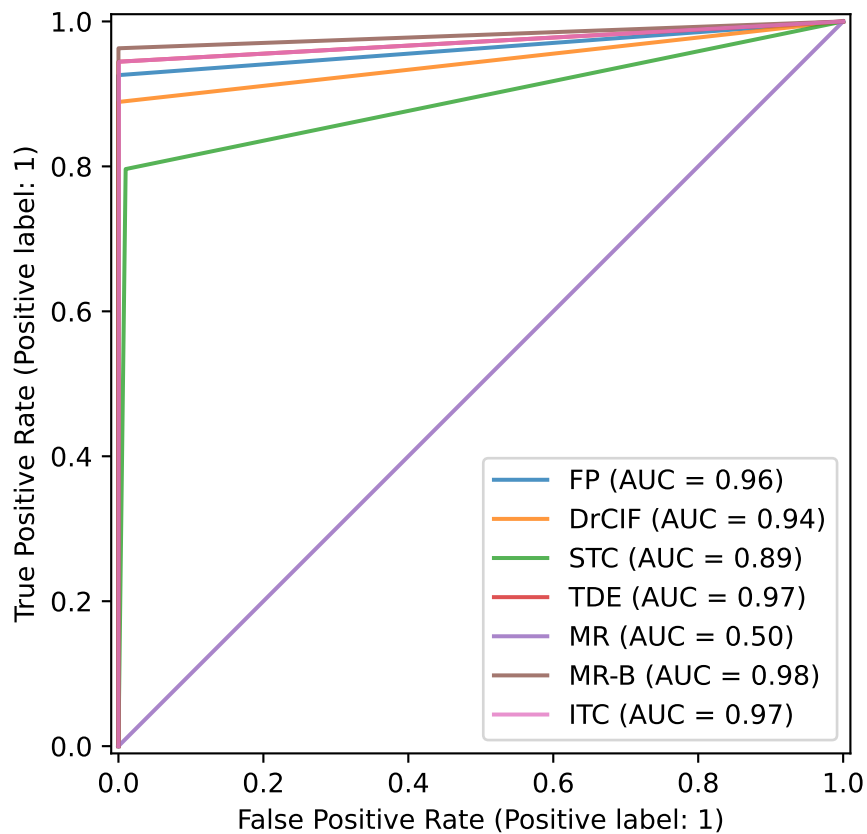
Roc Curve for Operation-wise performance
