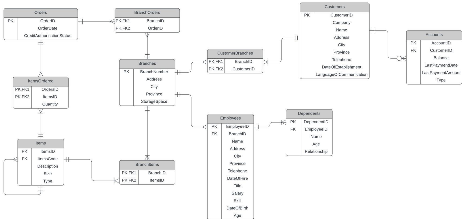
Figure 1: Milly Bonka's ER Diagram using Lucidchart.
