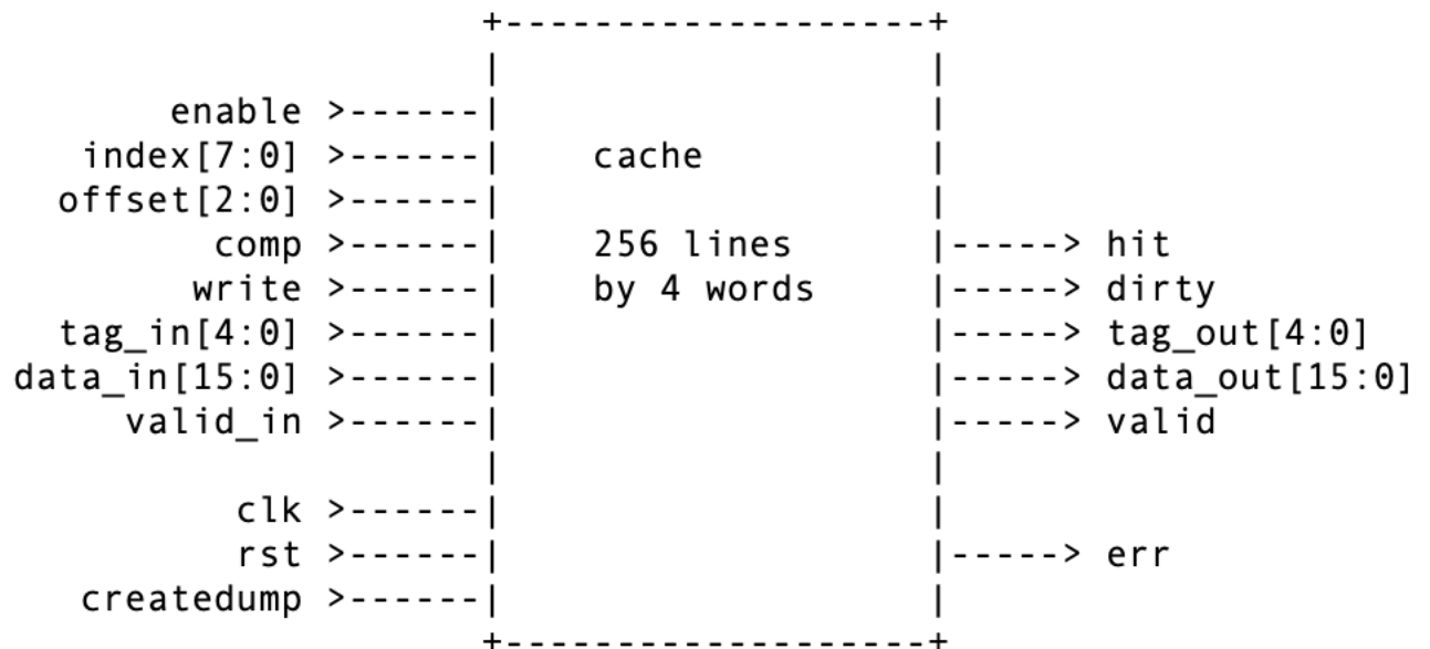
Figure 3: External Cache Interface
