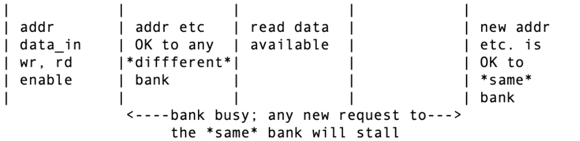
Figure 2: Timing
