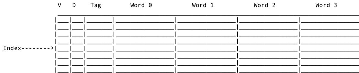
Figure 3: External Cache Interface
