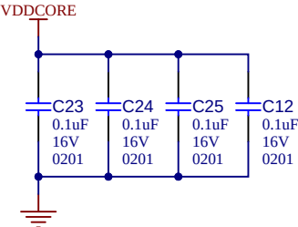
VDDCORE Bypass Caps
