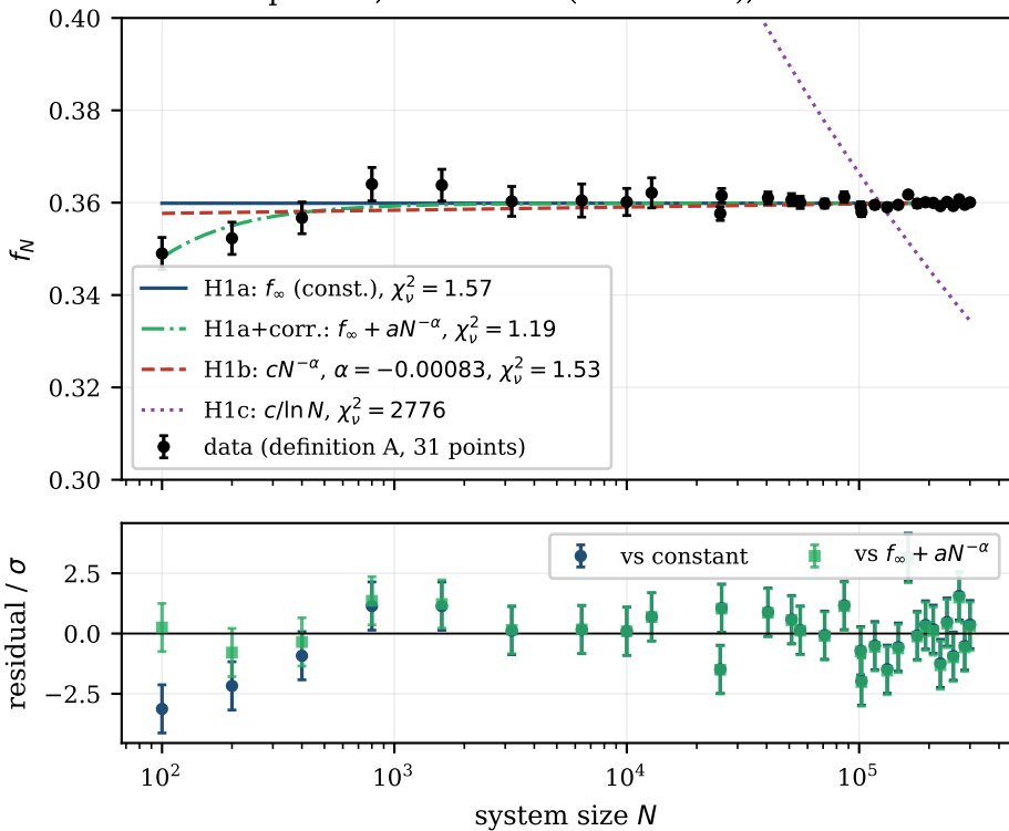
Model comparison, definition A (cumulative), N = 100 to 3 \times 10^5
