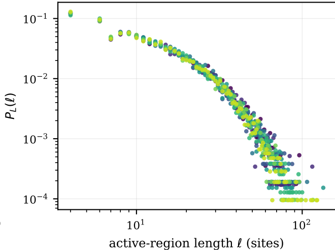
(b) log-log: straight \Rightarrow power law
