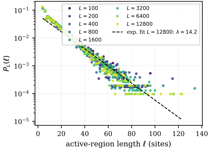
(a) semi-log: straight \Rightarrow exponential
