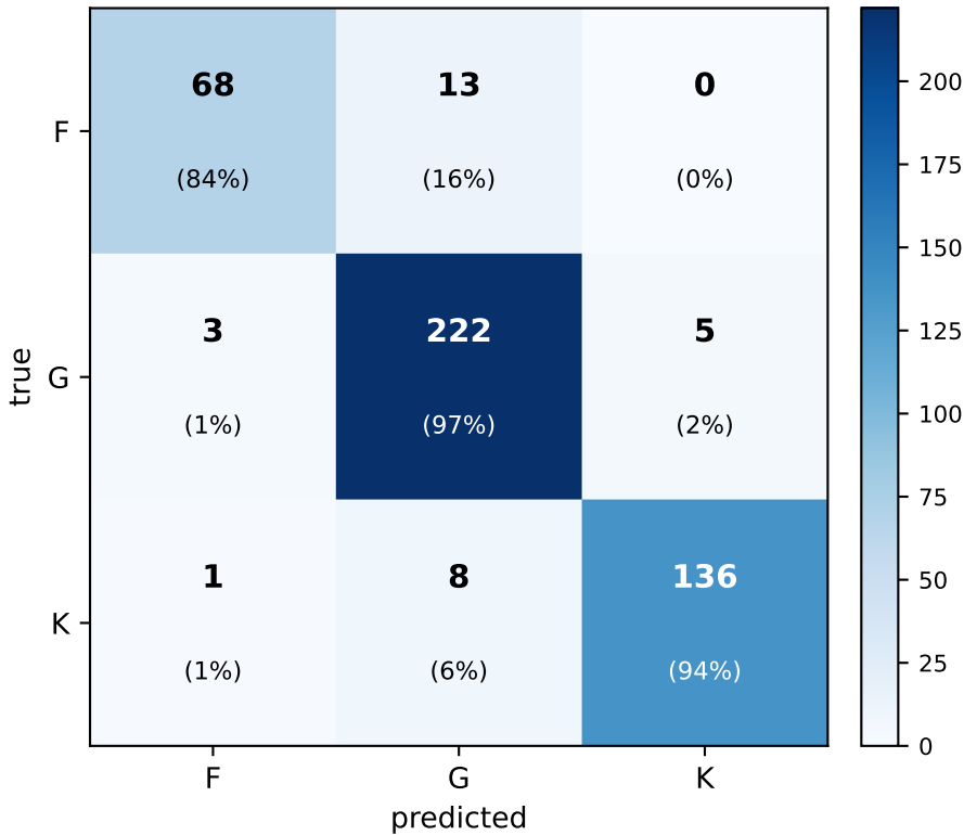
LightGBM (test set)
