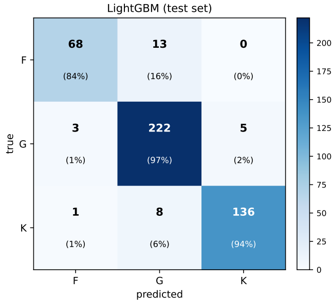
Figure 6: Held-out test confusion matrix. Rows are the true class and columns the predicted class, in F–G–K order.
