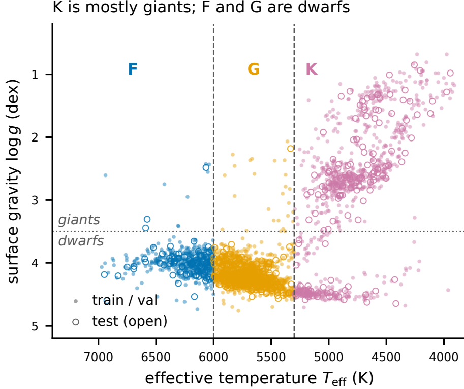
Figure 2: Kiel diagram of the labelled sample coloured by class. The F and G classes lie on the dwarf branch and the K class is dominated by giants; the dwarf cut is \log g = 3.5 .
