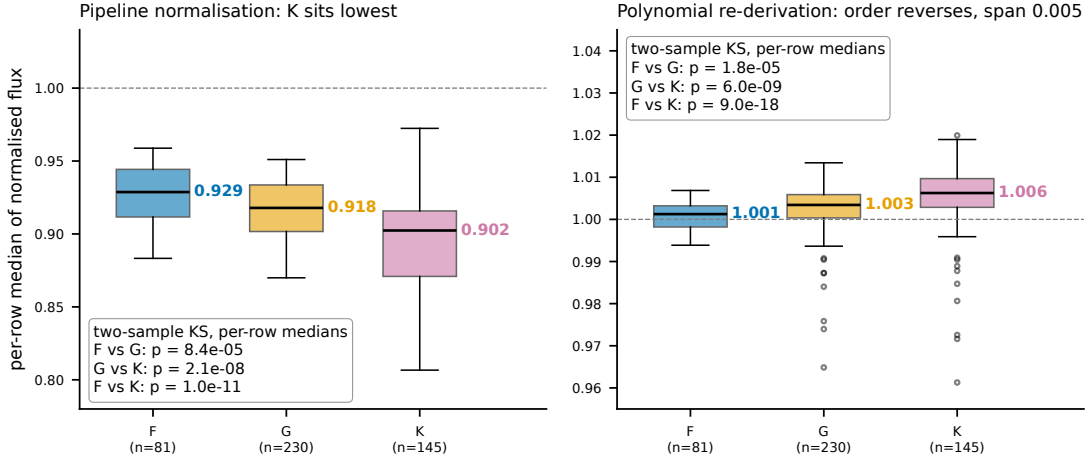
Figure 3: Per-row median of normalised flux outside the inter-chip gap by class on the test set, under the production normalisation (left) and after the polynomial re-normalisation (right). Class medians are given in Section 4.5; the numbers come from the same artifact as Table 7.
