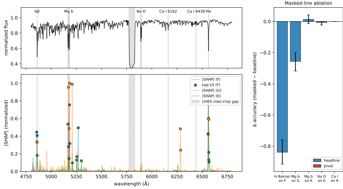
Figure 4: Top: per-bin median normalised spectrum of the G class with the diagnostic-line positions marked and the inter-chip gap shaded. Bottom: normalised mean |SHAP| per class (F blue, G orange, K green) with the ten largest bins of each class marked. Right: \Delta A (change in per-class accuracy, that is recall) for the headline and pivot pairs from the primary ablation run (production continuum, linear-interpolation fill), with 95 percent bootstrap intervals; the same quantities with their random-window p -values are in Figure 1 and Table 3.
