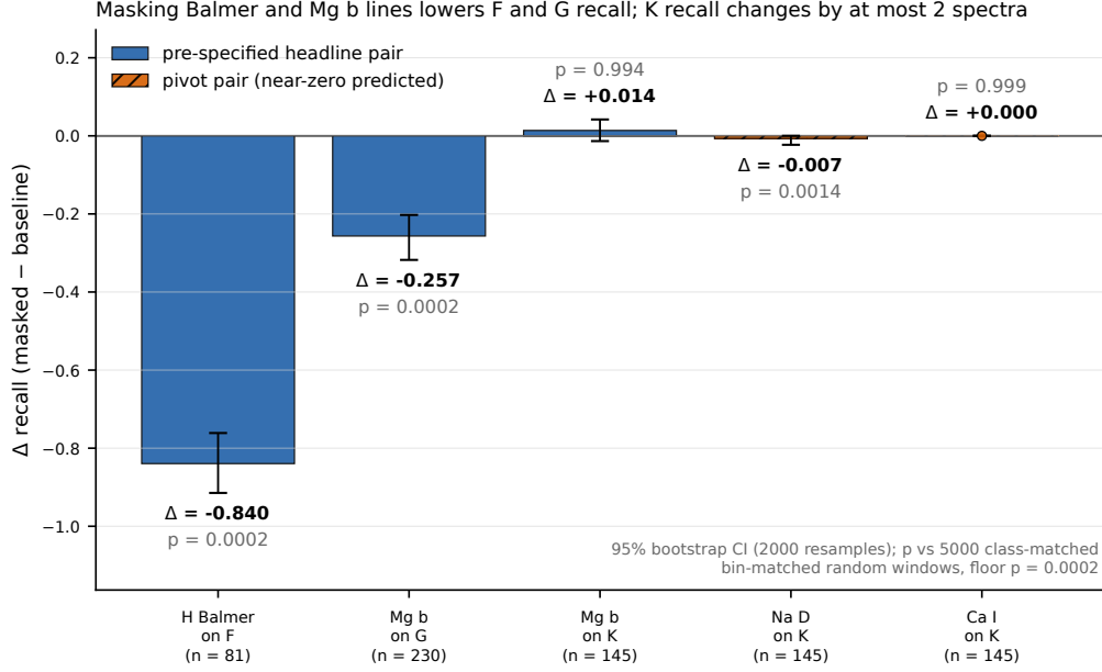
Figure 1: Change in class recall \Delta A_k^{(\mathcal{L})} for the headline (solid) and pivot (hatched) pairs in the primary configuration (production continuum, interpolation fill). Error bars are 95 percent bootstrap intervals (2000 resamples); each bar is annotated with \Delta A and the Monte Carlo p -value against 5000 class-matched, bin-matched random windows (floor 2.0 \times 10^{-4} ). The K bars are small but not exactly zero in rows (Section 4.3); the values match Table 3.
