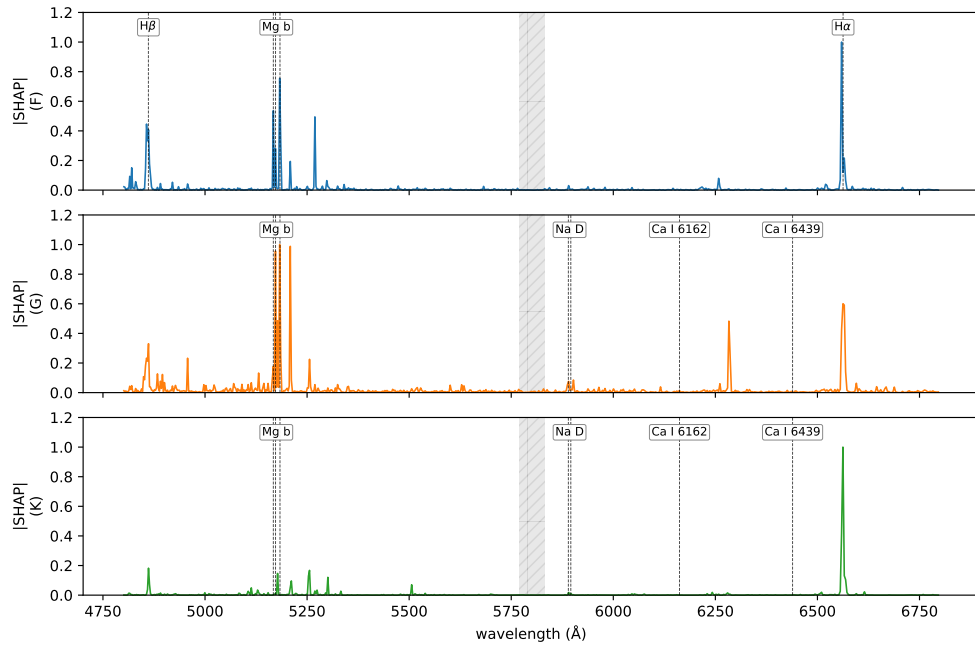
Figure 5: Per-class SHAP overlay with the inter-chip gap shaded.
