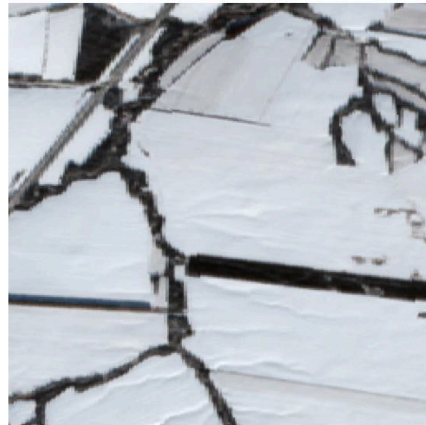
GT optical
