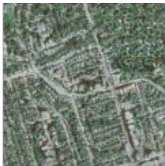
Pix2Pix
