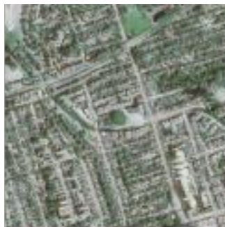
CycleGAN
