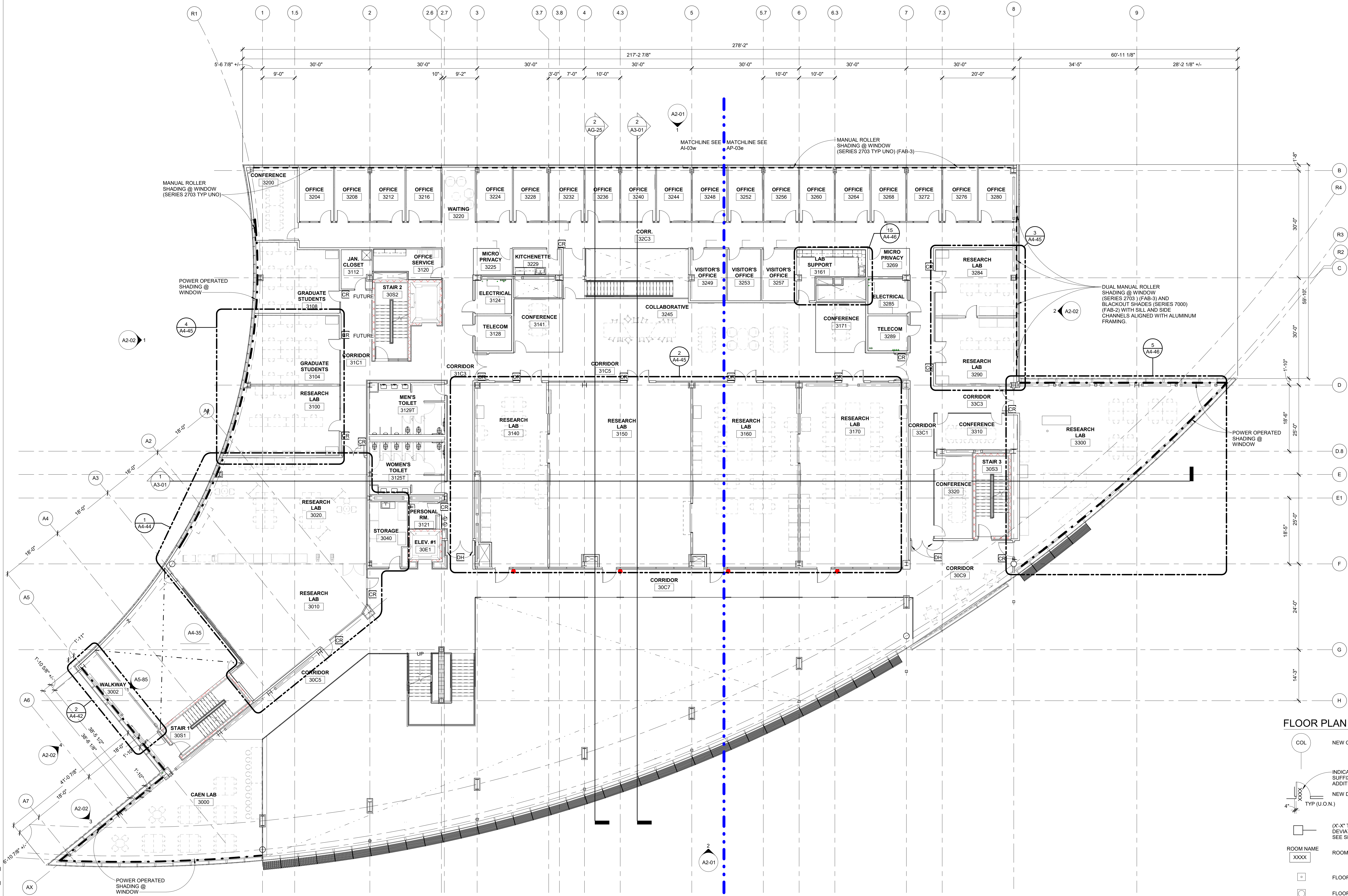
COMPOSITE THIRD FLOOR PLAN SCALE: 3/32" = 1'-0"
