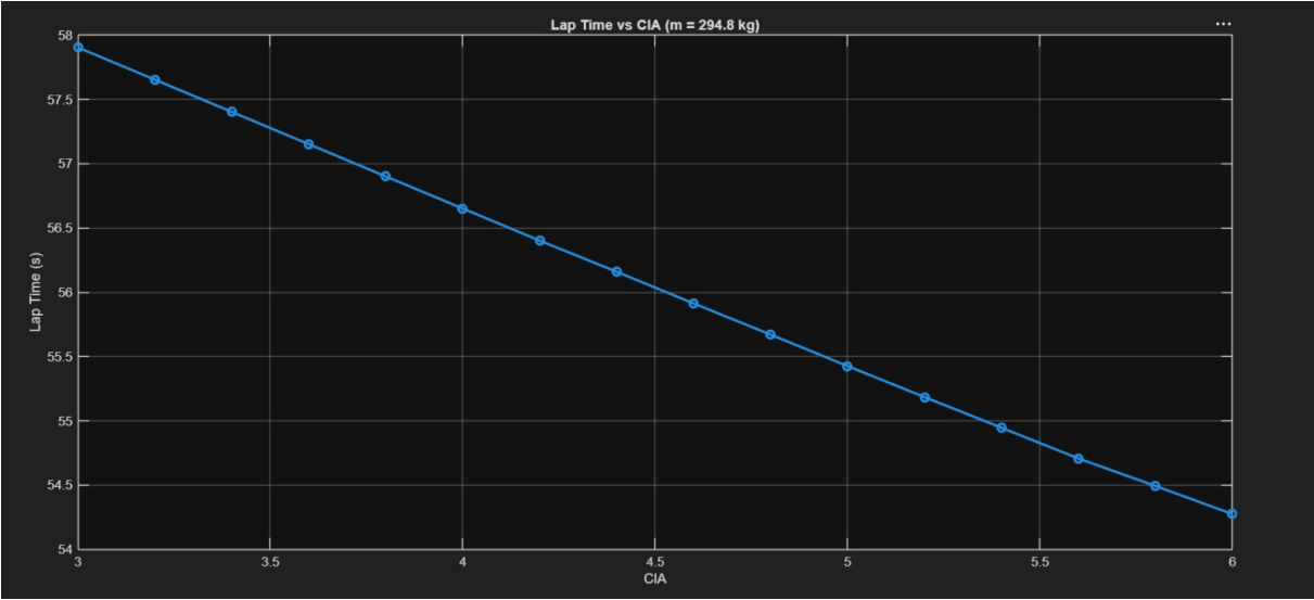
Lap time vs. CIA (m = 294.8 kg)
