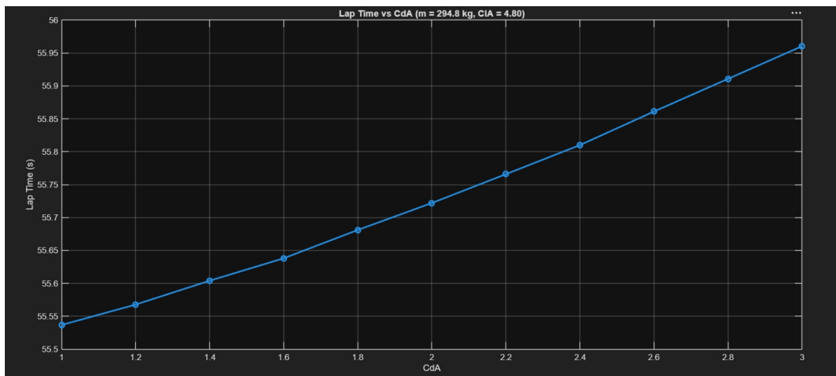
Lap time vs. CdA (m = 294.8 kg, CIA = 4.80)
