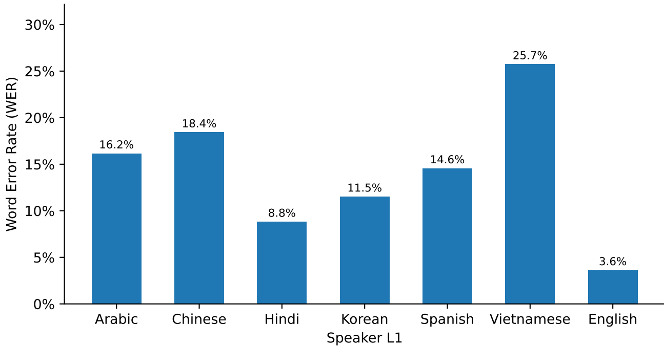
Whisper baseline WER by speaker L1
