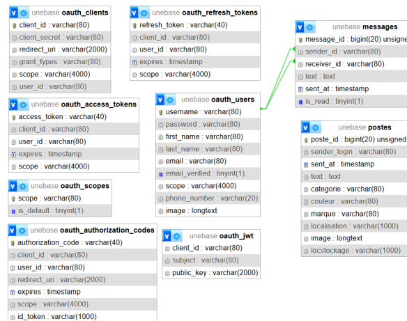
Figure 3: Database architecture
