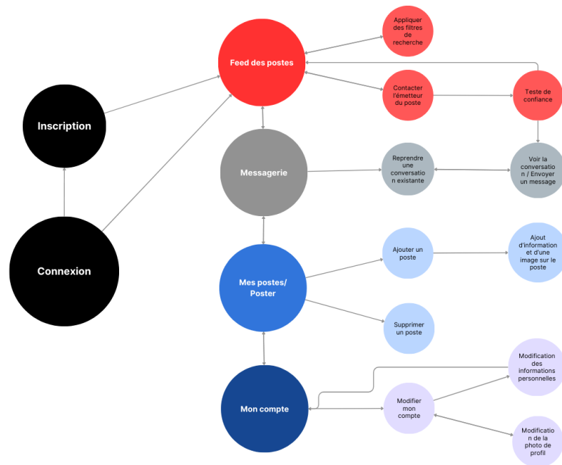
Figure 2: Client architecture
