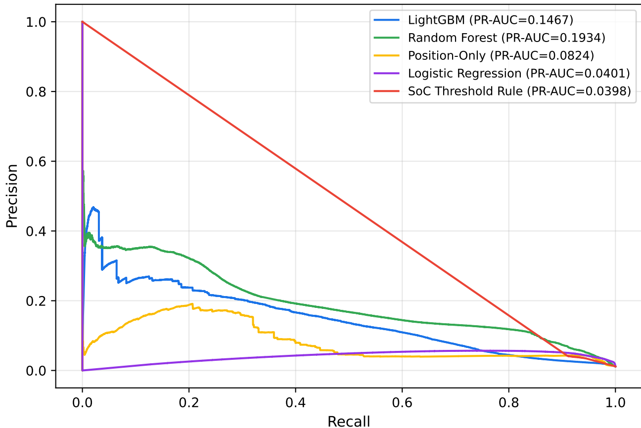
Precision-Recall Curves across Full Unfiltered Test Folds
