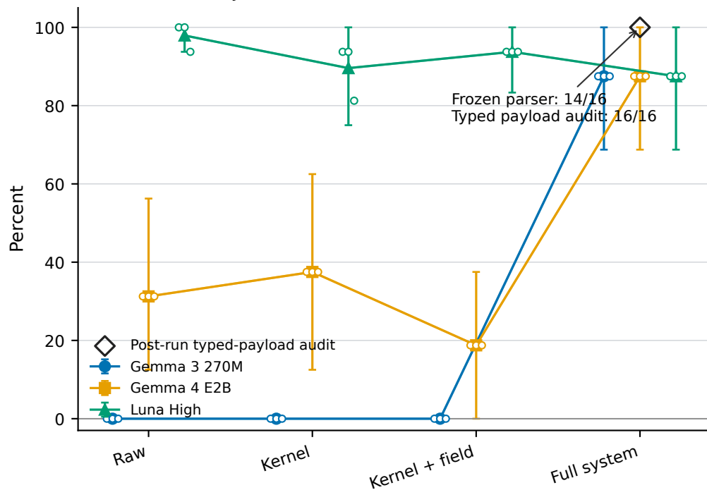
A. Objective numeric tolerance (16 cases)
