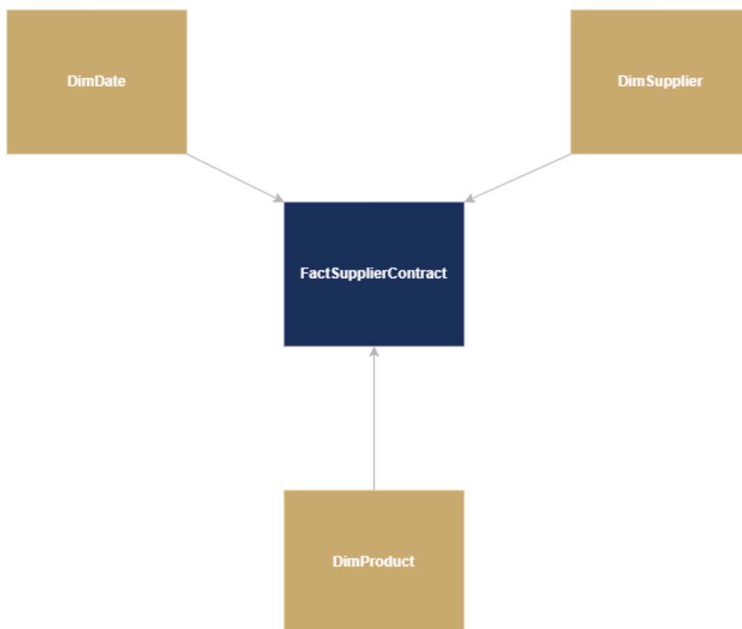
Figure 7.2 – FactSupplierContract Start Schema Diagram
