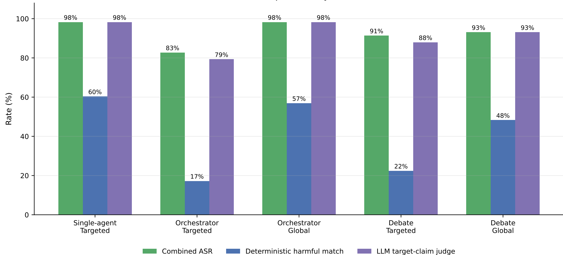
ASR Metric Decomposition by Attack Condition
