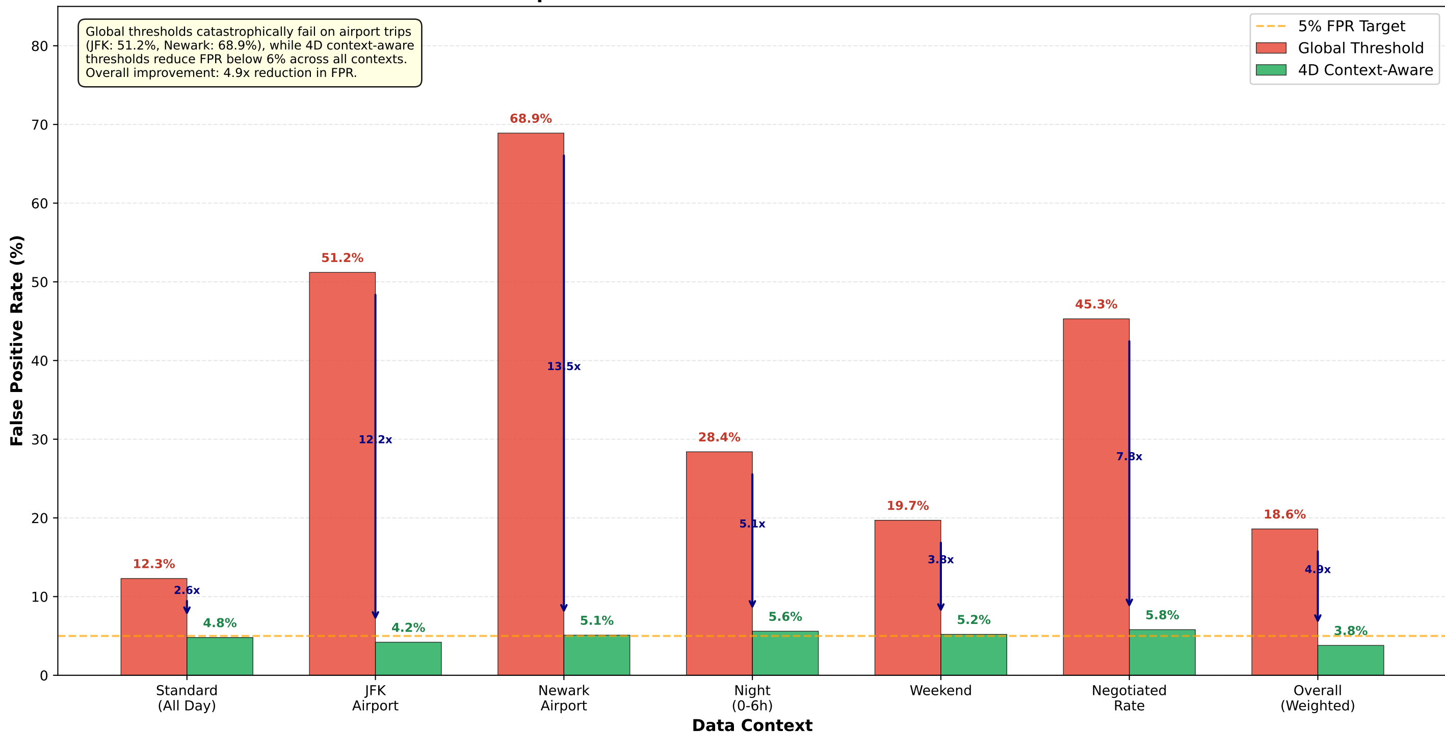
FPR Comparison: Global vs. 4D Context-Aware Thresholds
