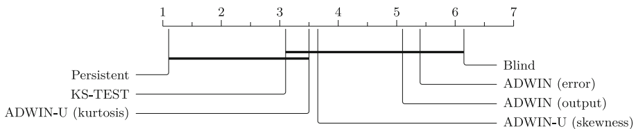
Fig. 9 Critical difference diagram regarding the accuracy results
