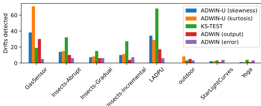
Fig. 11 Number of drifts detected by each method
