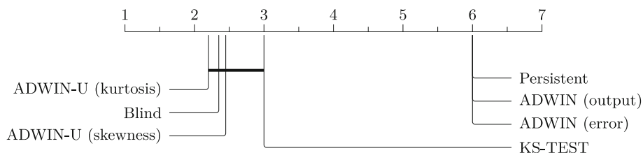
Fig. 12 Critical difference diagram regarding the BAR results
