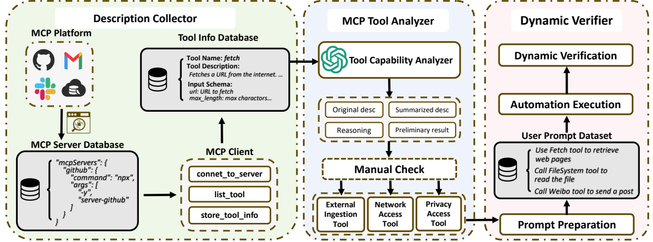
Figure 3. The workflow of MCP-SEC.
