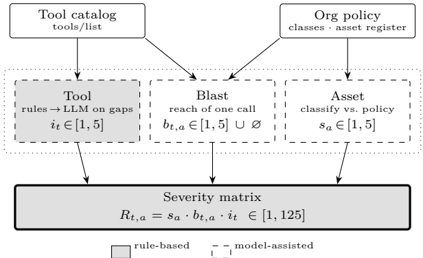
Fig. 1. Static (design-time) scoring. Two documents—the server’s advertised tool catalog and the organization’s written policy—feed three scanners, each producing exactly one primitive: tool impact i_t over the T tools, asset sensitivity s_a over the A assets, and blast radius b_{t,a} over all T \times A pairs. Their product is the severity matrix. Since i and s are each indexed by a single dimension, b is what distinguishes a cell from others in its row; b_{t,a} = \emptyset marks a tool that cannot reach an asset and removes the cell. The organization states no severity number: s_a is derived by classifying each asset against the policy’s own classes.
