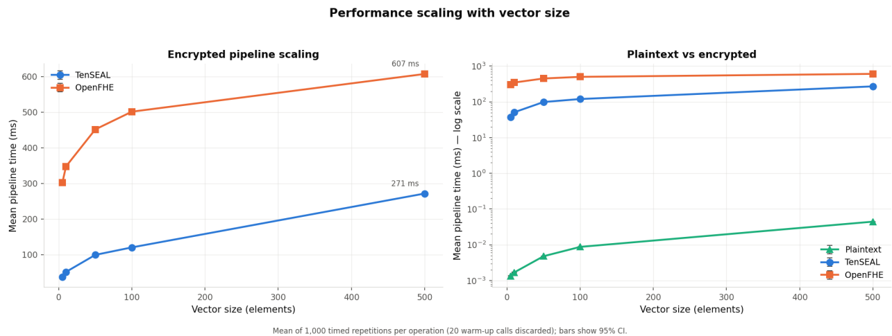
Figure 4: Pipeline time versus vector size. Left: the encrypted libraries. Right: all three on a log scale.
