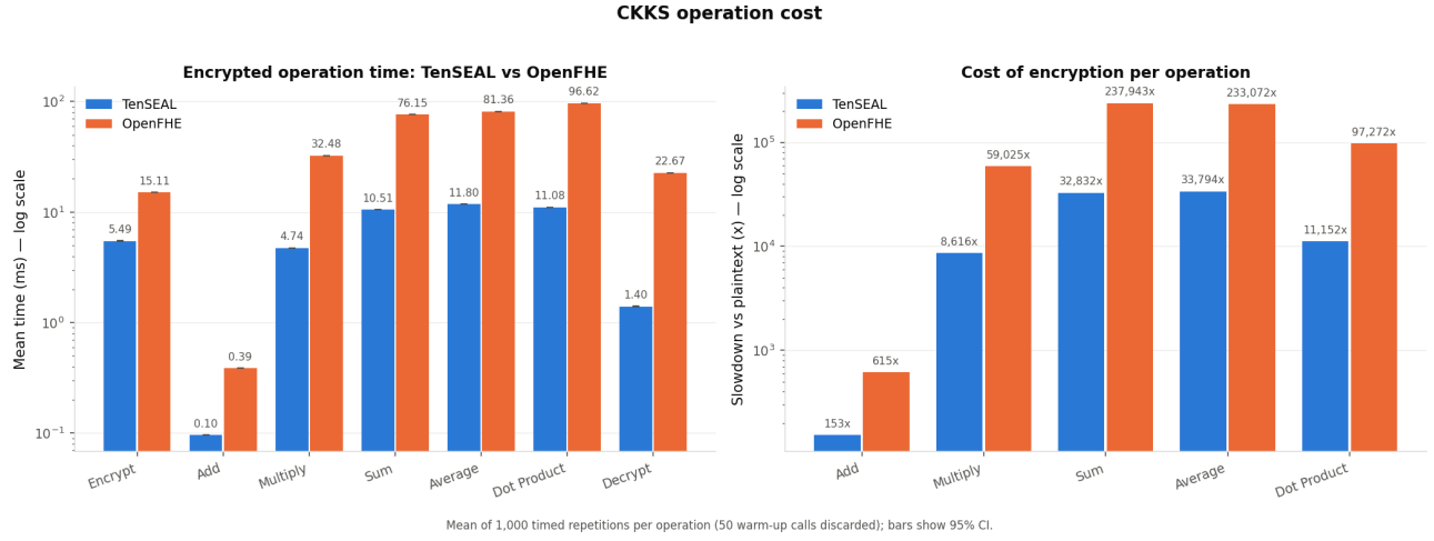
Figure 1: Mean time per operation, and slowdown versus plaintext. Bars carry 95% confidence intervals; note the log scale on both panels.
