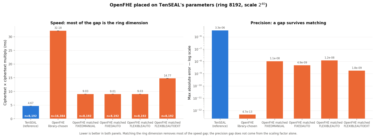
Figure 5: OpenFHE placed on TenSEAL’s parameters. Lower is better in both panels.
