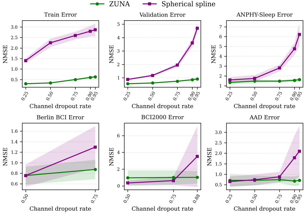
Figure 1: Zyphra ZUNA
