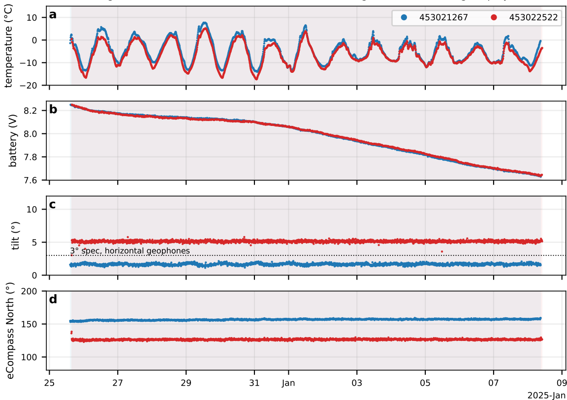
Dronning Maud Land, Antarctica: state of health from DigiSolo.LOG (shading: deployments)
