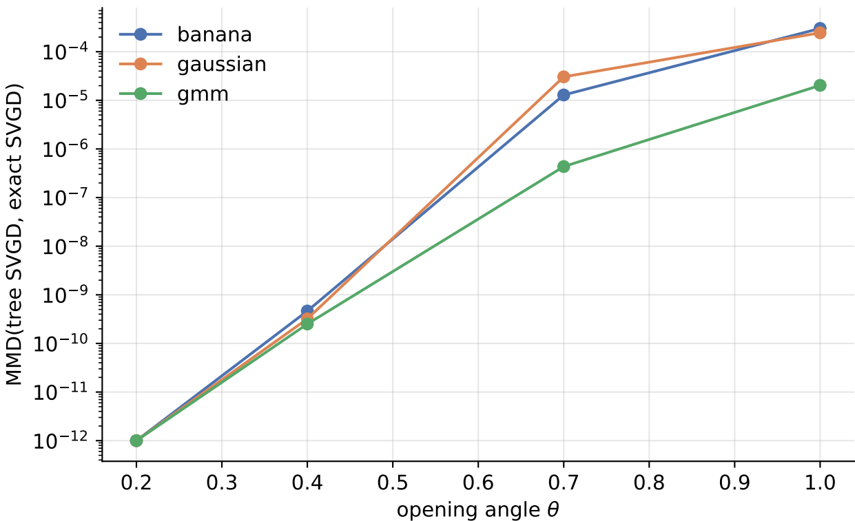
Tree-accelerated SVGD vs. exact, across theta
