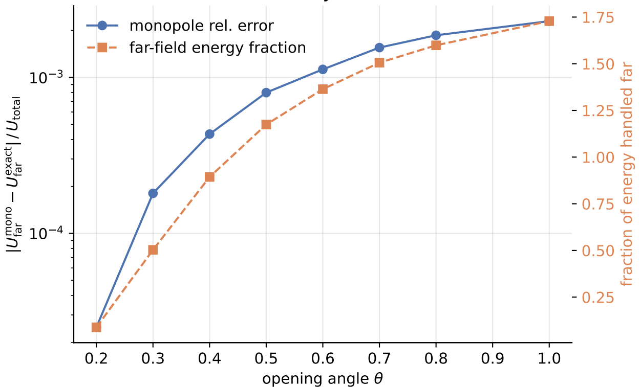
Dehnen MAC accuracy vs. cost (N=20000)
