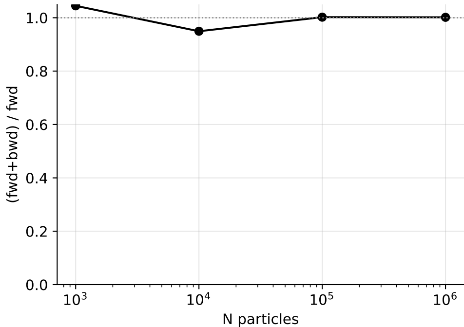
Autodiff overhead ratio
