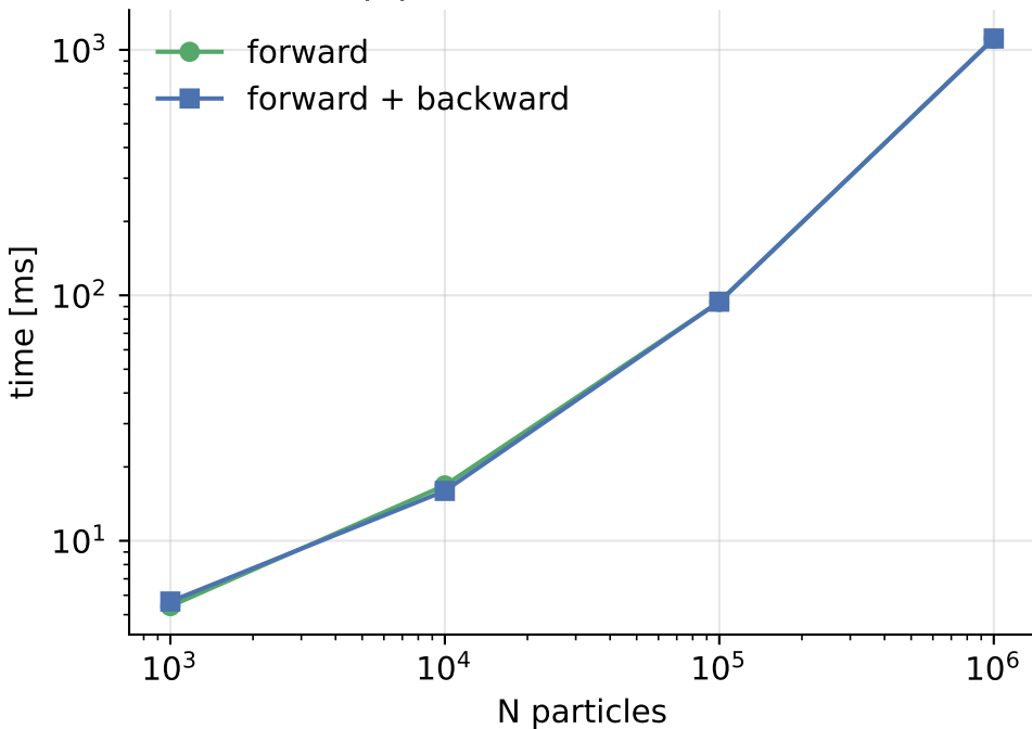
KD-tree pipeline: build + kNN + reduce
