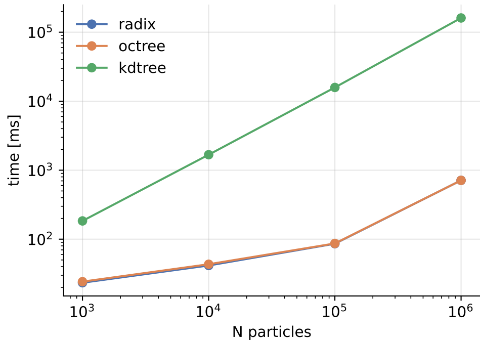
Dual-tree traversal
