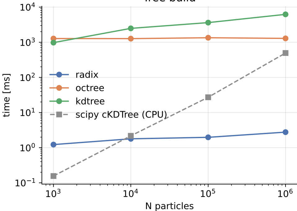
Tree build
