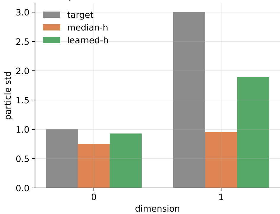
Dispersion: learned vs. median heuristic
