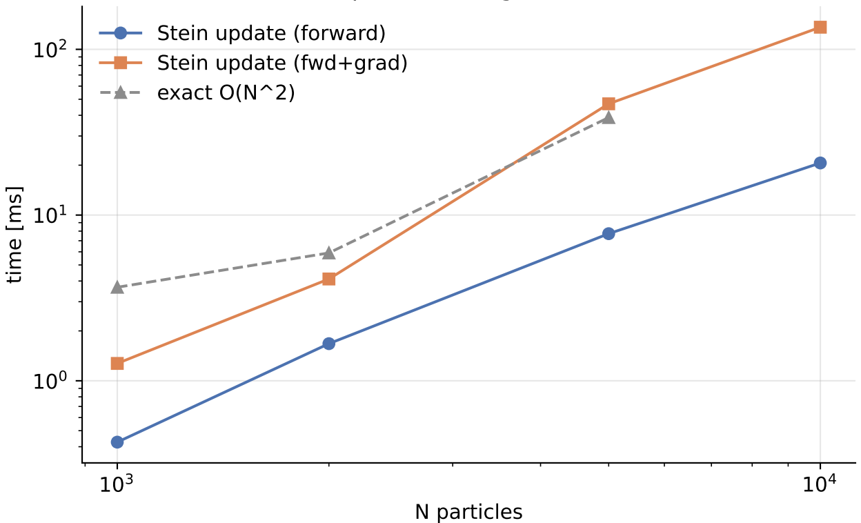
Tree-accelerated SVGD update scaling (NVIDIA GeForce RTX 2080 Ti)
