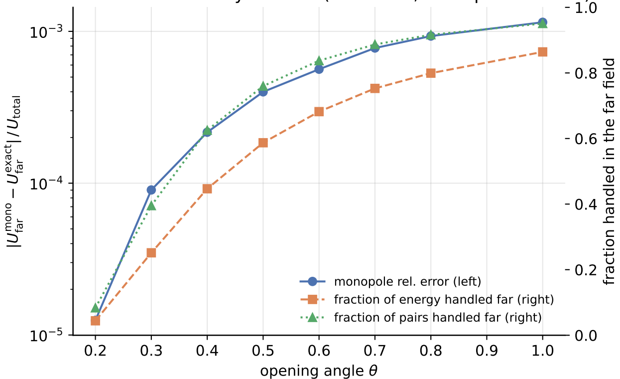
Dehnen MAC accuracy vs. cost (N=20000, monopole far field)
