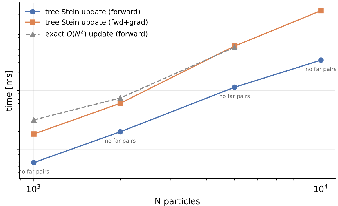
Stein update cost, d=5, KD-tree
