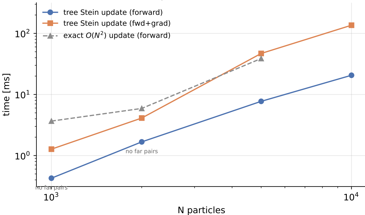
Stein update cost, d=3, radix
