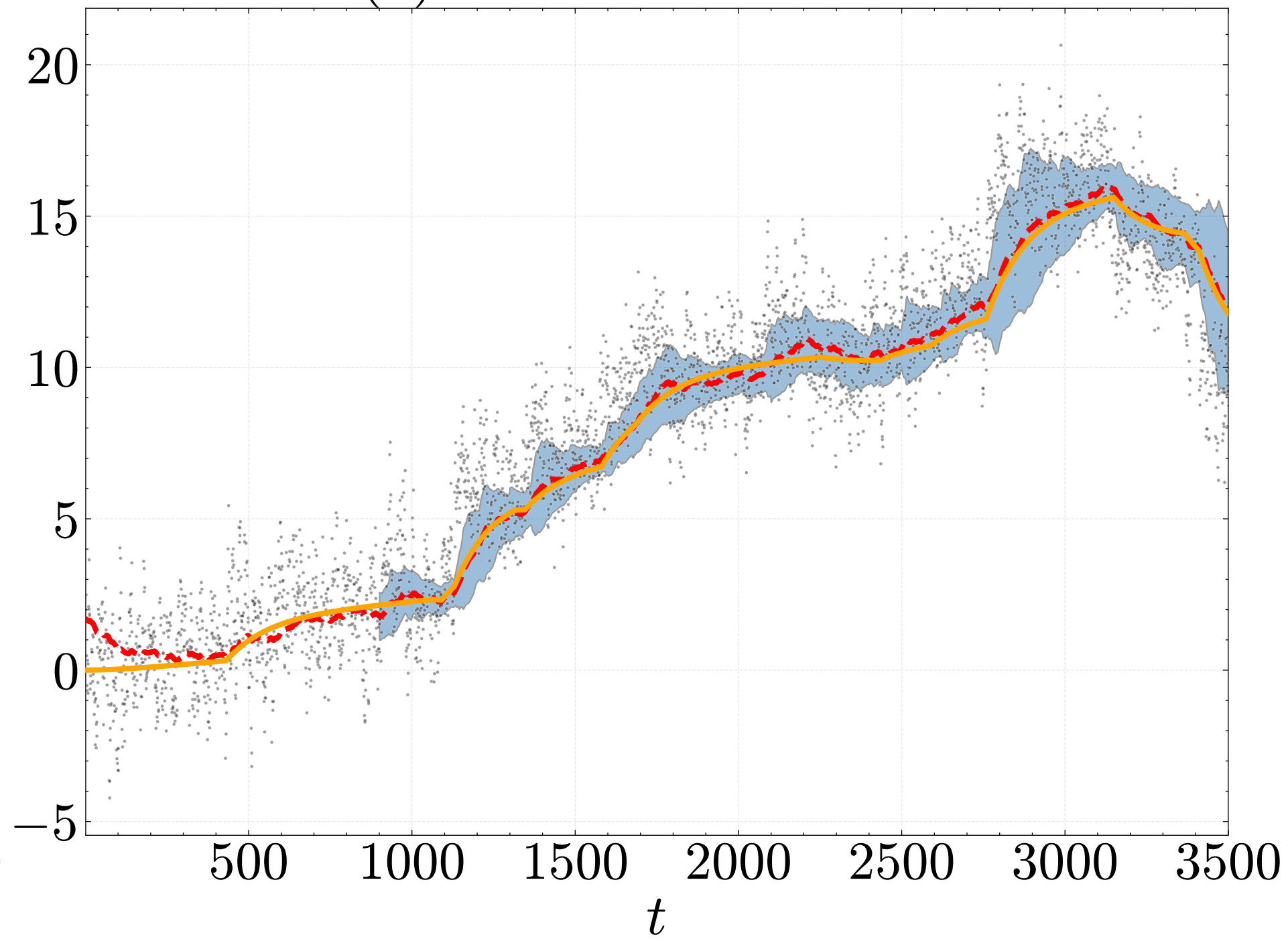
AR(1) with trend and shocks
