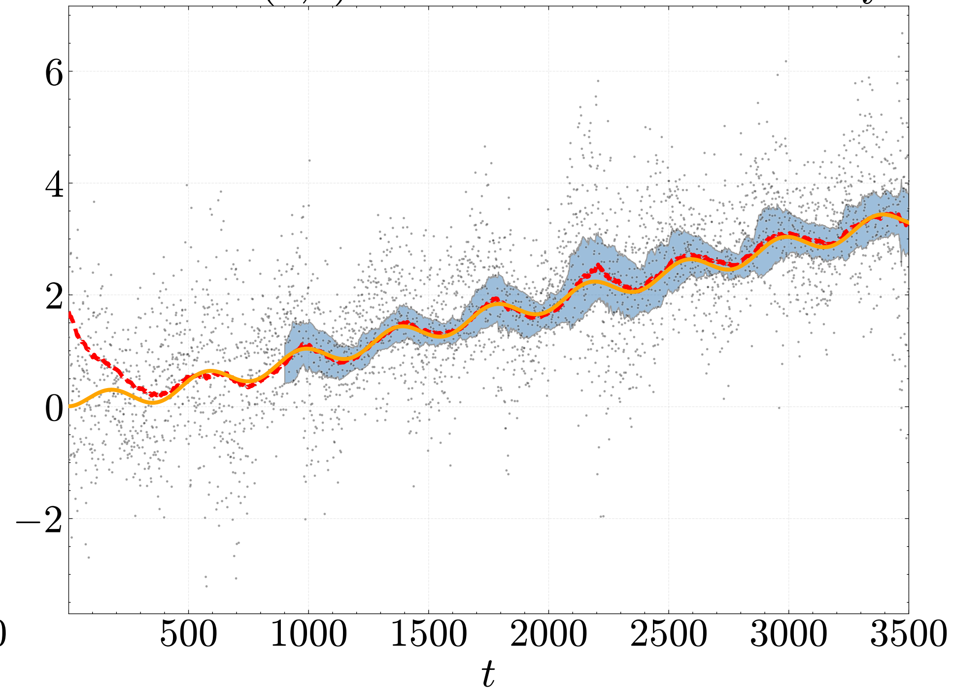
GARCH(1,1) with trend and seasonality
