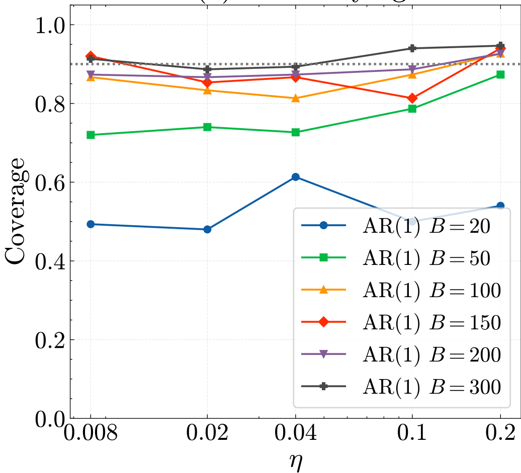
AR(1) with varying B
