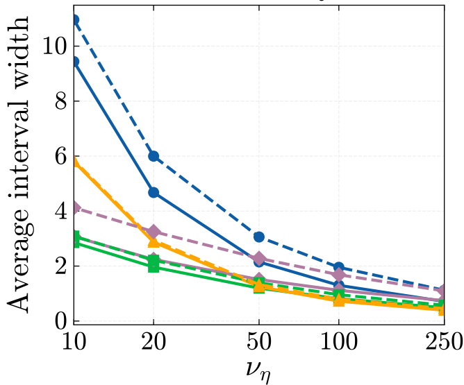
Stationary
