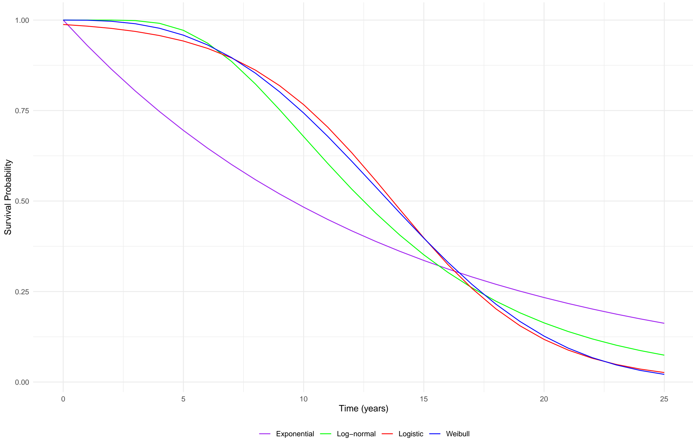
Fitted Survival Curves for Death
