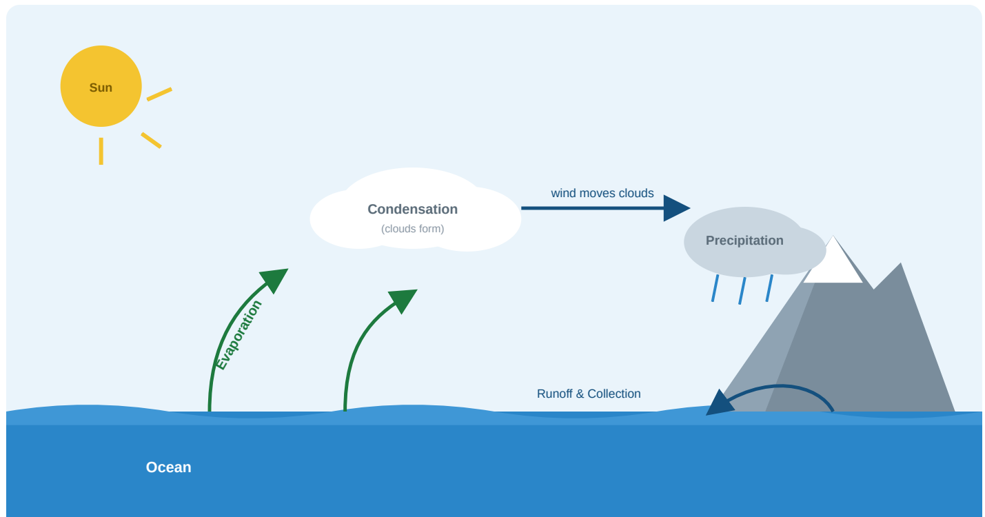
Figure 3.2 — The Sun powers the water cycle: evaporation, condensation, precipitation, and collection.
