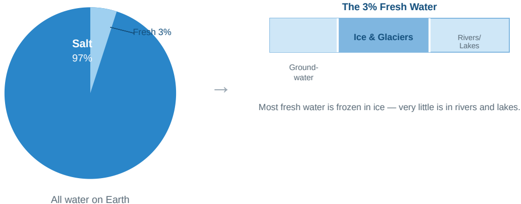
Figure 3.1 — Almost all water is salty. Only a little is fresh, and most fresh water is frozen. (The fresh slice is drawn bigger so you can see it.)
