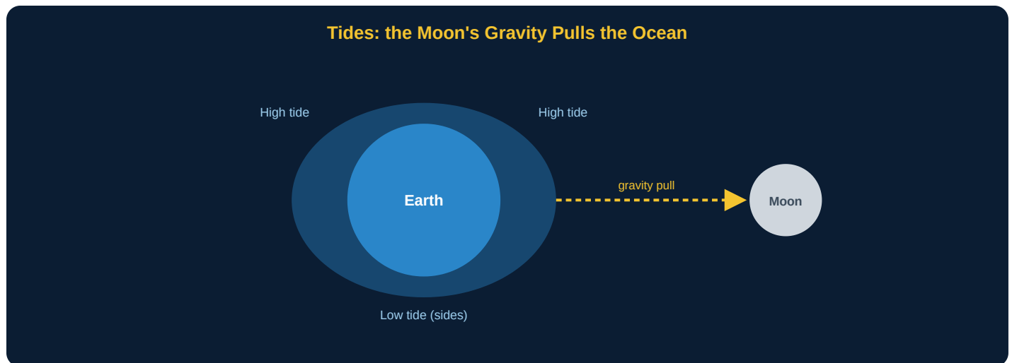
Figure 3.4 — The Moon's gravity pulls the ocean into bulges. Under a bulge = high tide.
