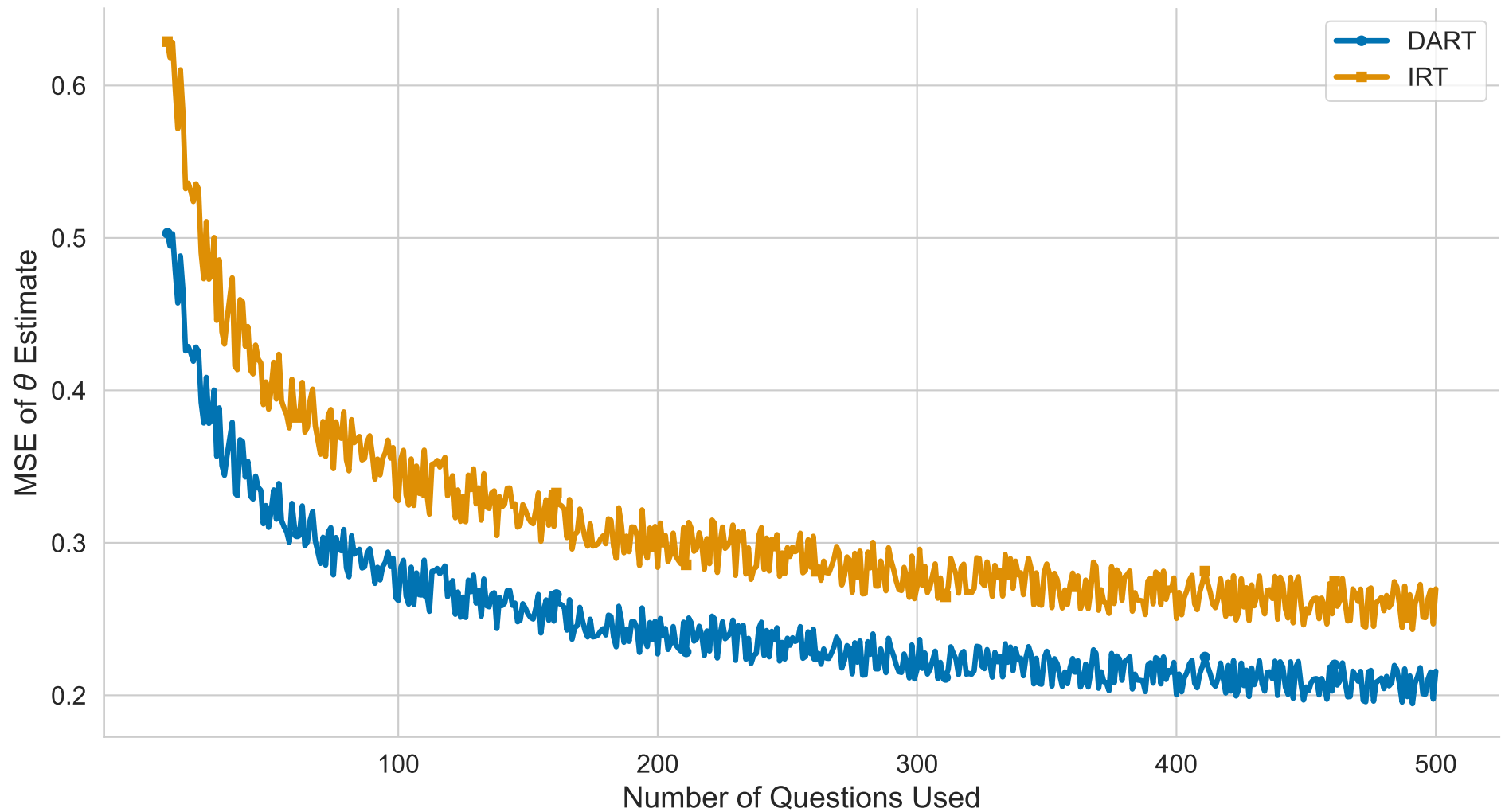
Efficiency Comparison between DART and IRT on Math500
