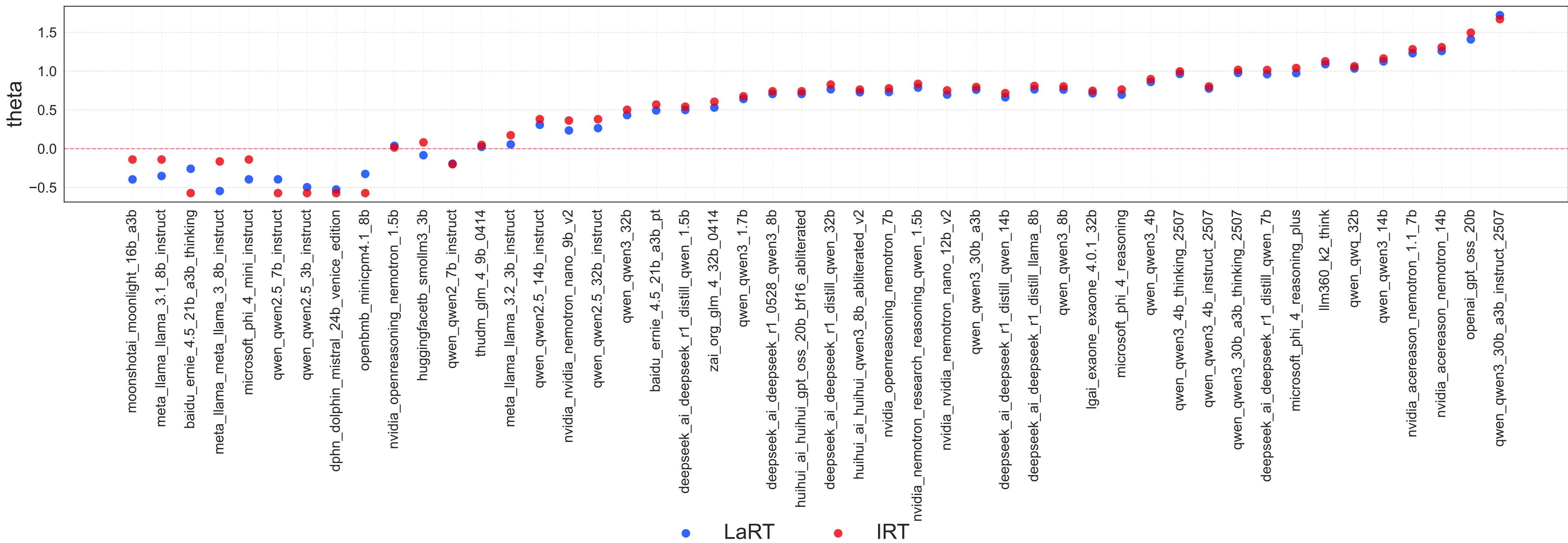
LaRT and IRT on AIME24 for One-Shot Models
