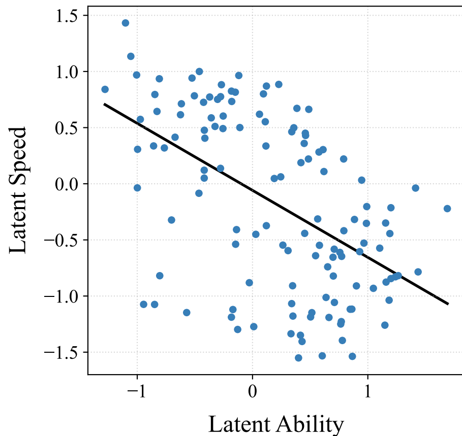
AIME 2025, \rho = -0.81
