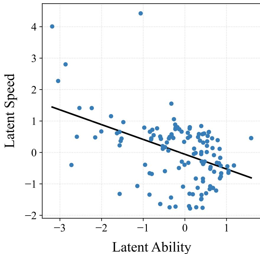
AIME 2024, \rho = -0.75
