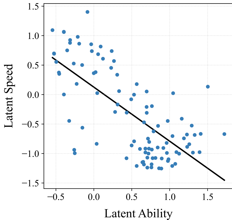
AIME 2024, \rho = -0.75
