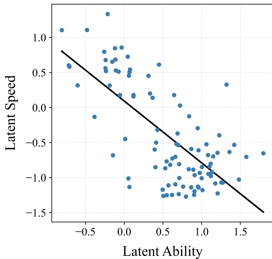
AIME 2025, \rho = -0.81
