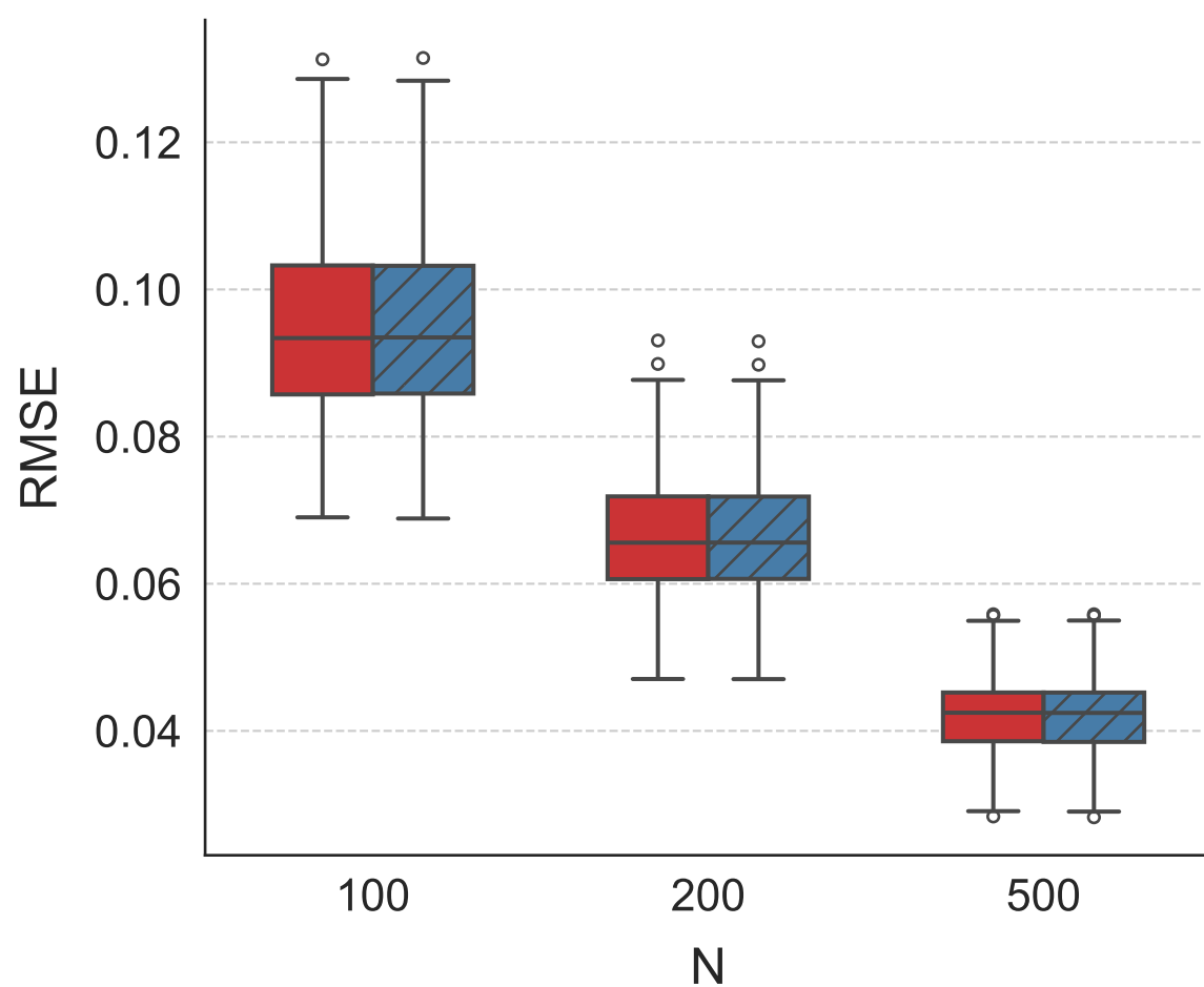
lambda
