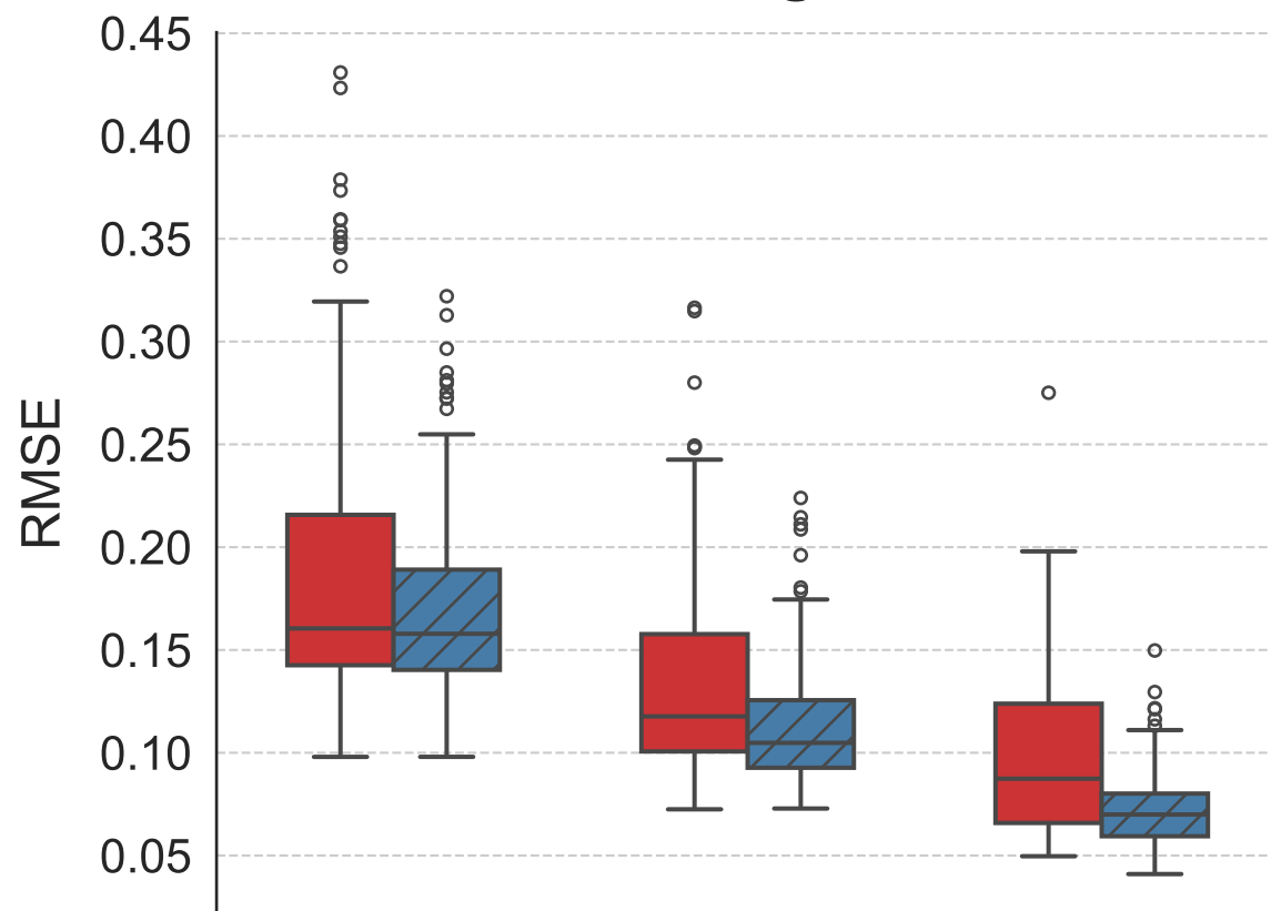
lambda
