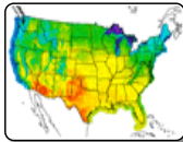
US Temperatures
